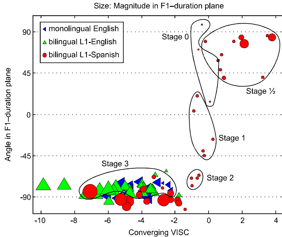
Figure 8.7 Plot of the F1–duration-plane angle and magnitude, and the converging-VISC contrast for the English /i/–/ɪ/ boundaries from logistic regression models calculated for each participant. Groupings indicate participants at different stages of the hypothesised indirect developmental path, and participants on the direct developmental path.
