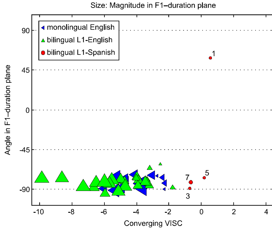
Figure 10.1 Plot of the F1–duration-plane angle and magnitude, and the converging-VISC contrast for the English /i/–/ɪ/ boundaries from logistic regression models calculated for each L1-English participant and for L1-Spanish L2-English participant bs075 at LOR = 1, 3, 5, and 7 months (numbers on plot indicate LOR in months).
