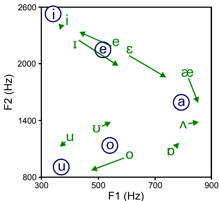
Figure 1.1 Blue symbols within circles: Mean F1–F2 values for Peninsular Spanish monophthongs measured in the middle of vowels in isolated words. Data from Martínez Celdrán (1995), averaged over five male and five female speakers. Green symbols with arrows: Mean F1–F2 values for Canadian English nominal monophthongs and phonetic diphthongs measured at the beginning and end of isolated vowels. Data from Nearey & Assmann (1986), averaged over five male and five female speakers.
