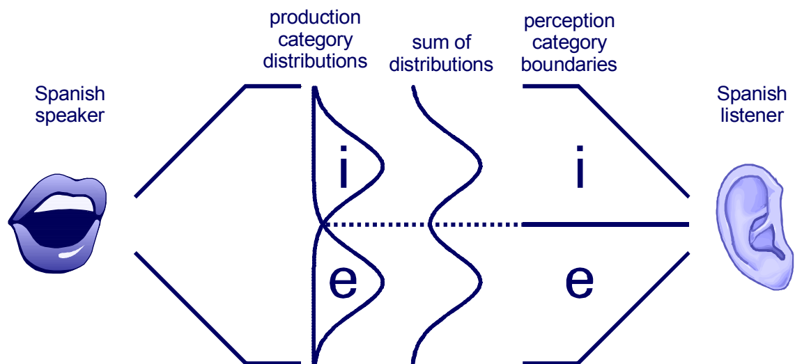
Figure 1.2 A stylised one-dimensional illustration of L1 speech perception learning, see text. The dotted line represents the location of a boundary which optimally categorises the Spanish vowel productions.
