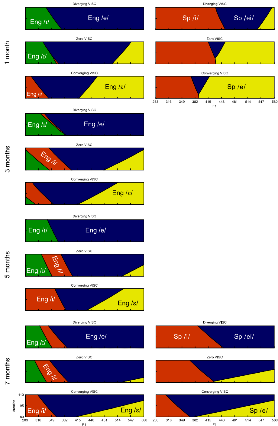
Figure 10.8 Territorial maps based on logistic regression models fitted to Participant bs069's vowel identification data at LOR = 1, 3, 5, and 7 months.
