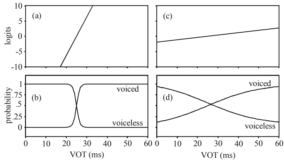
Figure A7.5 Linear slopes in the logistic space (a and c) and the corresponding sigmoidal curves in the probability space (b and d) for contrast coefficient values of 1.256 logits/ms (a and b) and 0.079 logits/ms (c and d).
