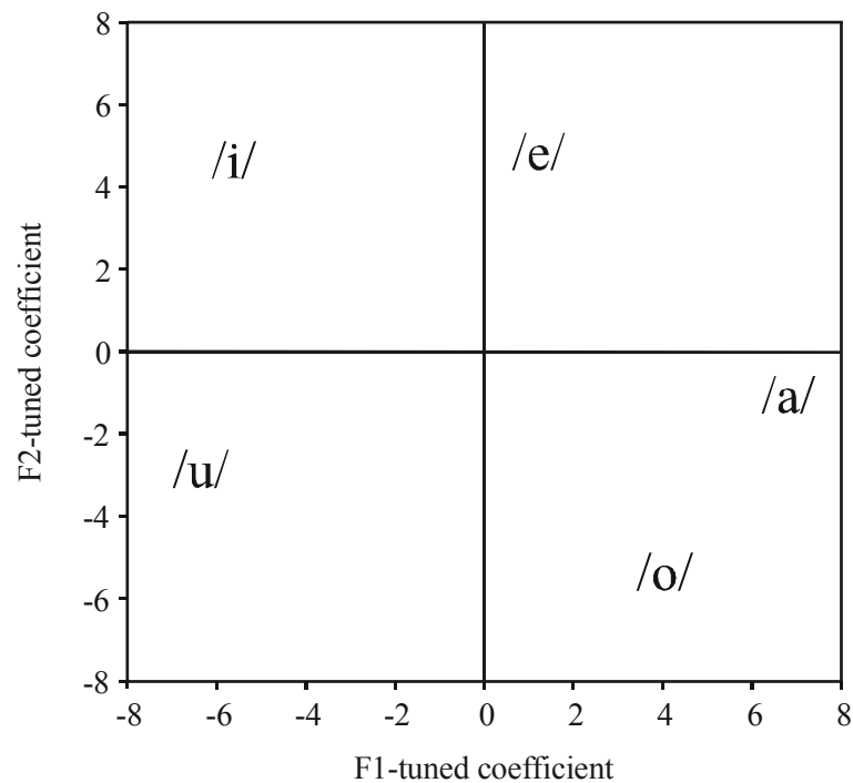
Figure A7.2 Plot of estimated values of stimulus-tuned logistic regression coefficients for Model 1b fitted to the vowel perception data from Álvarez González.
