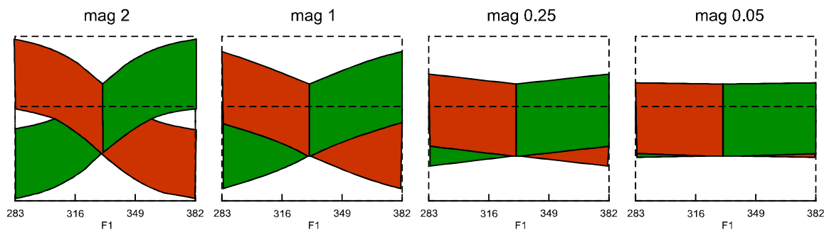
Figure 8.3 Example probability surface plots illustrating different magnitudes for the English /i/–/ɪ/ boundary. Boundary angle is fixed at -90^\circ .
