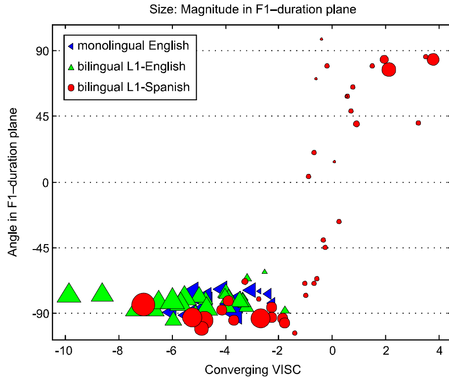
Figure 8.5 Plot of the F1–duration-plane angle and magnitude, and the converging-VISC contrast for the English /i/–/ɪ/ boundaries from logistic regression models calculated for each participant.
