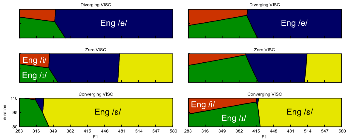
Figure 8.9 Example territorial maps for participants assigned to Stage 1 of the hypothesised indirect developmental path. Left: bs083, /i/-/ɪ/ angle +20.5°, converging VISC -0.69
