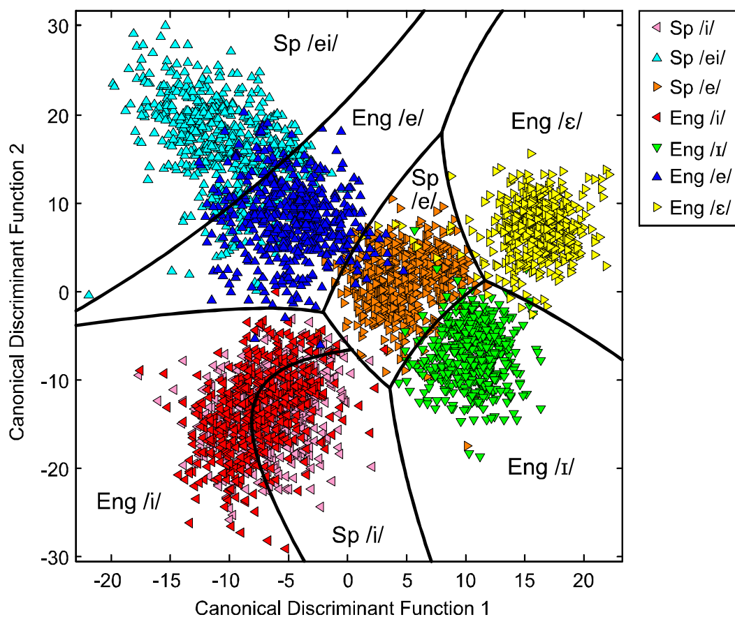
Figure 7.1 Location of L1-English and L1-Spanish speakers' vowel productions in the Function 1 – Function 2 space of a CDFA trained on both L1-English and L1-Spanish speakers' vowel production data.
