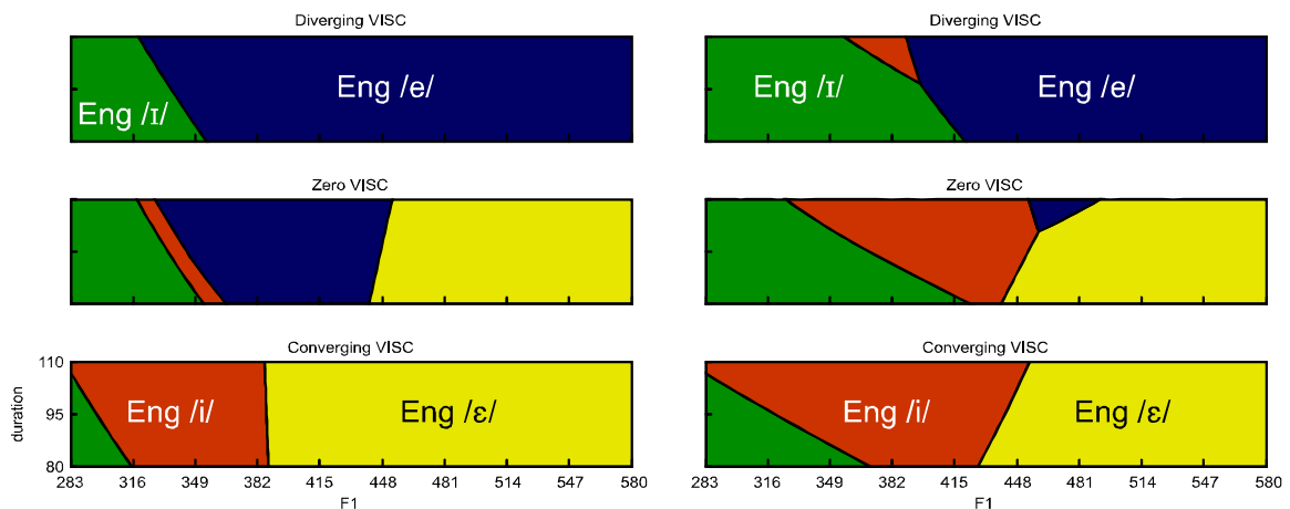
Figure 8.8 Example territorial maps for participants assigned to Stage \frac{1}{2} of the hypothesised indirect developmental path.
