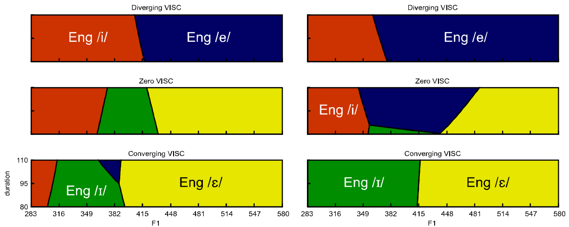
Figure 8.11 Example territorial maps for participants assigned to Stage 3 of the hypothesised indirect developmental path. Left: bs067, /i/-/ɪ/ angle -85.7^\circ , converging VISC -2.31
