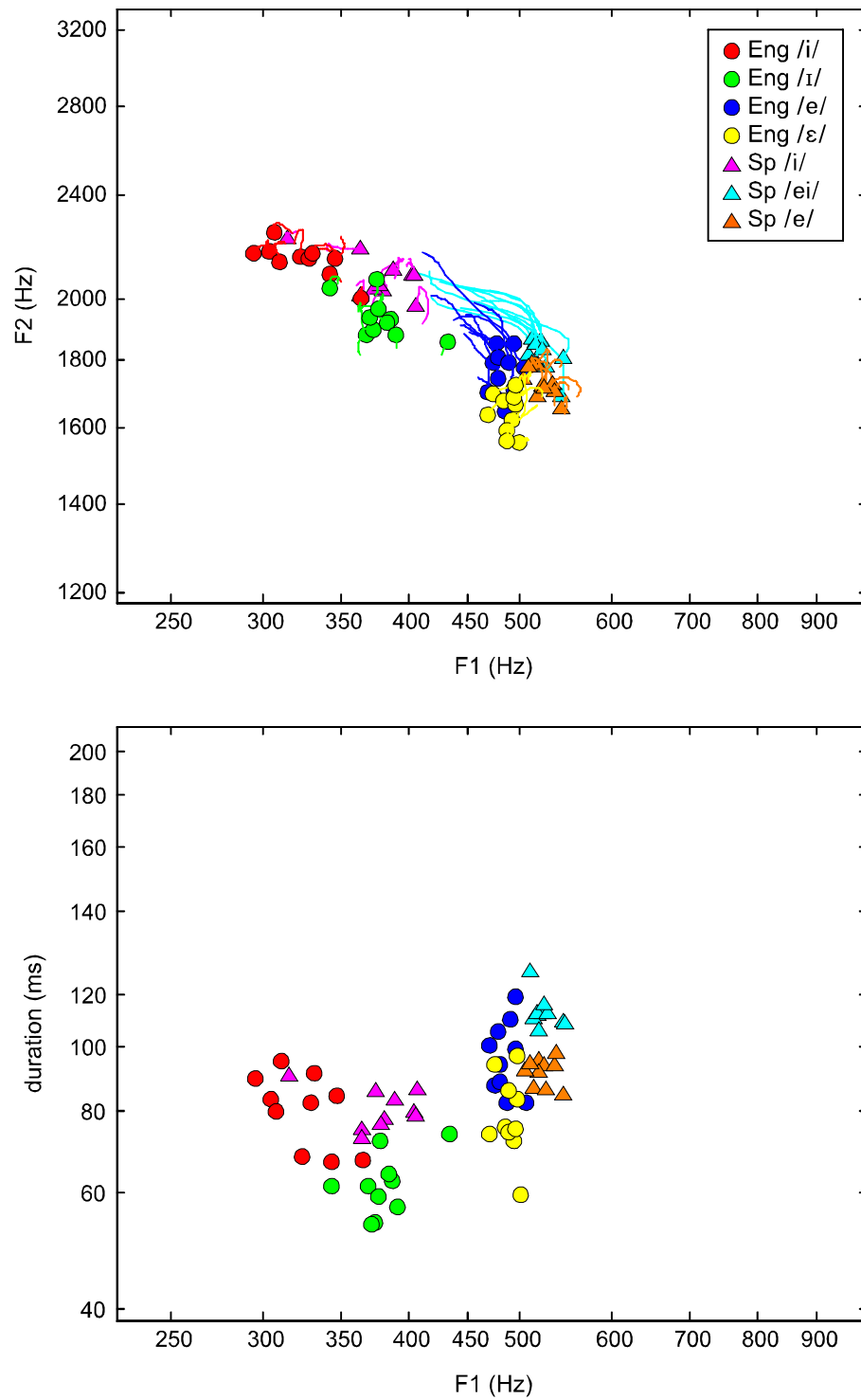
Figure 9.4 Example of Production Pattern D, English /ɪ/ produced with higher-F1-lower-F2 and shorter duration than English /i/ (Participant bs023).
