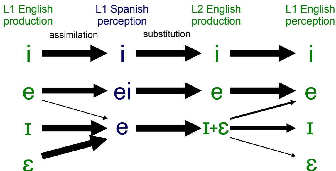
Figure 3.7 Predicted pattern of assimilation of L1-English vowel productions to L1-Spanish vowels, substitution of L1-Spanish vowels for L2-English production, and perception of L2-English productions by L1-English listeners. Predictions made on the basis of comparison of L1-English and L1-Spanish vowel production models. Arrow thickness indicates percentage of instances of vowel category on left perceived as vowel category on right (predicted percentages of less than 5% not shown).
