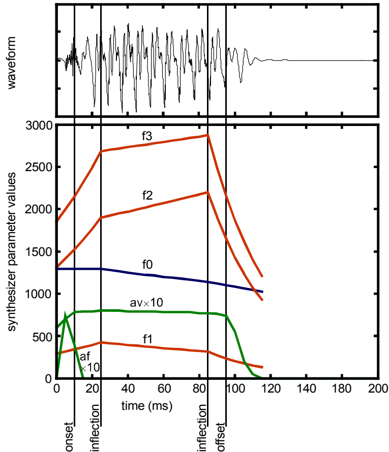
Figure 2.1 Sample variable parameter values used in the Klatt synthesiser. f1 , f2 , f3 are first, second, and third formants with values in Hertz, f0 is the fundamental frequency with values in tenths of Hertz, av and af are voicing and fricative amplitude with values in decibels (plotted at ten times the decibel values).
